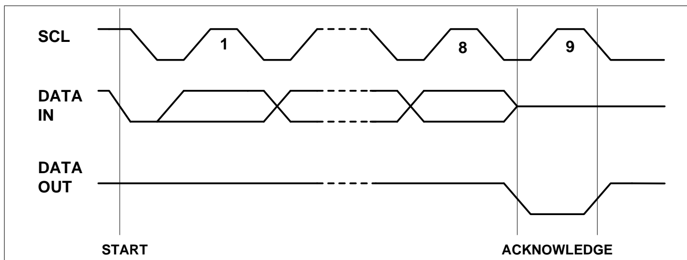
Figure 9. Output Acknowledge
