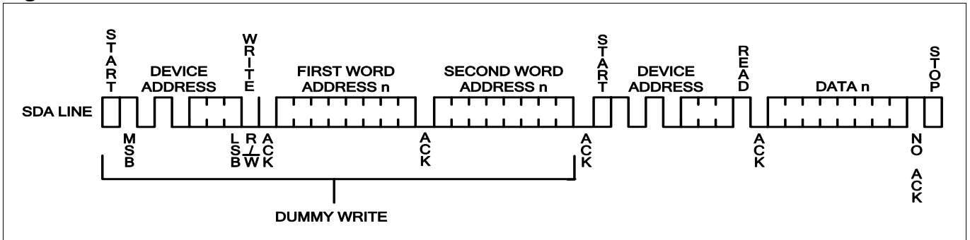
Figure 16. Random Read
