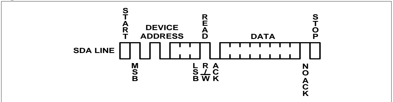
Figure 15. Current Address Read
