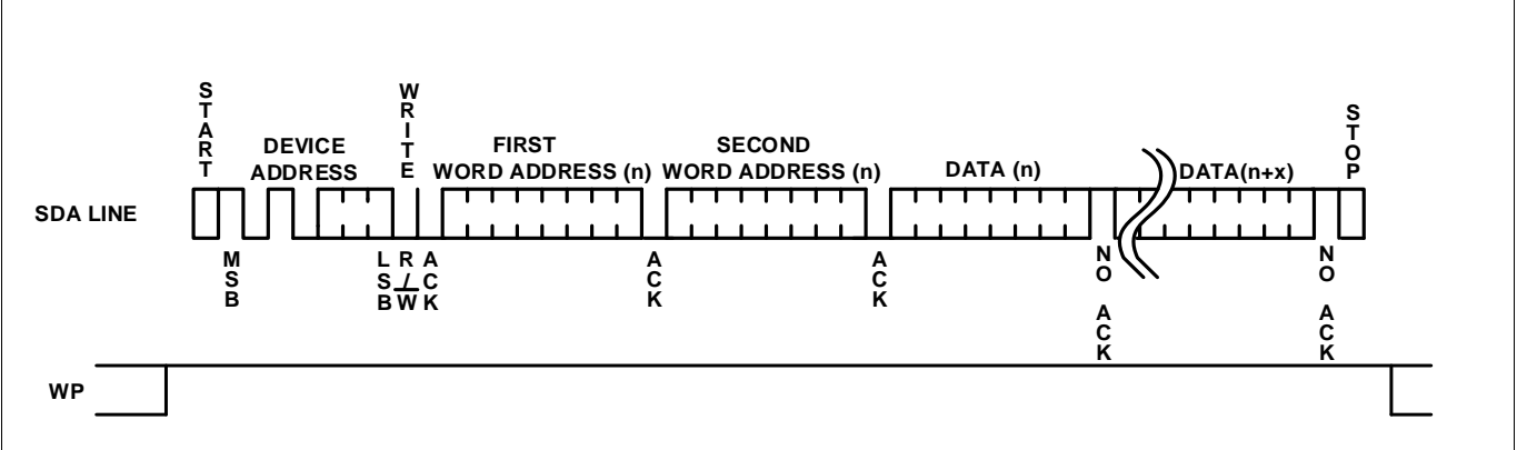
Figure 13. Write-Protect Condition
