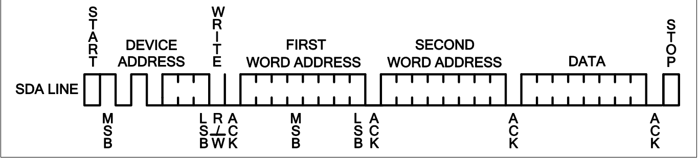
Figure 11. Byte Write
