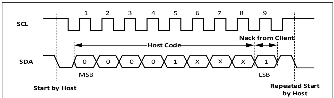
Figure 4. High-Speed Mode Entry Sequence
