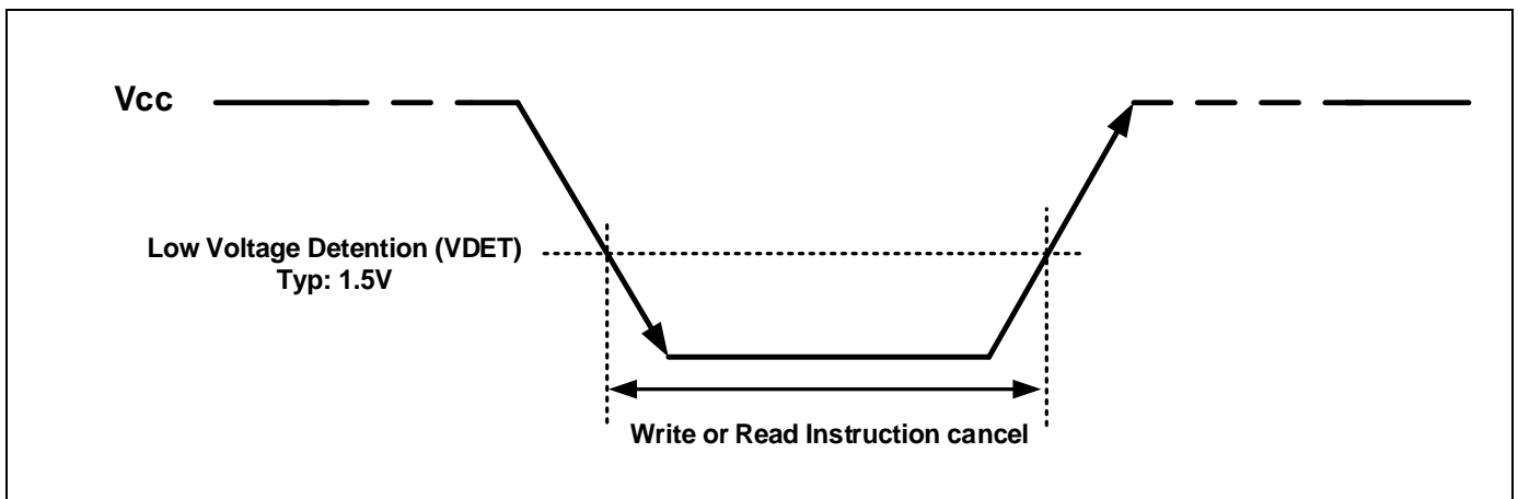
Figure 3. Operation during Low Power Supply Voltage
