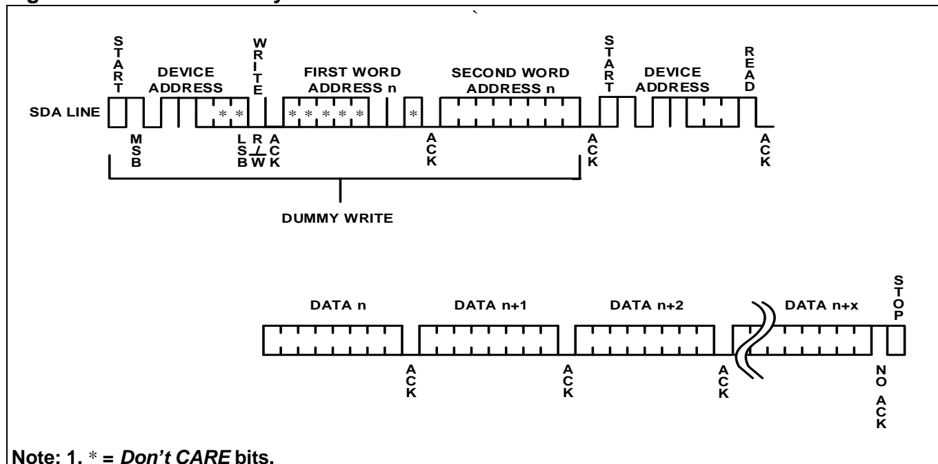
Figure 19. Read Security Sector
