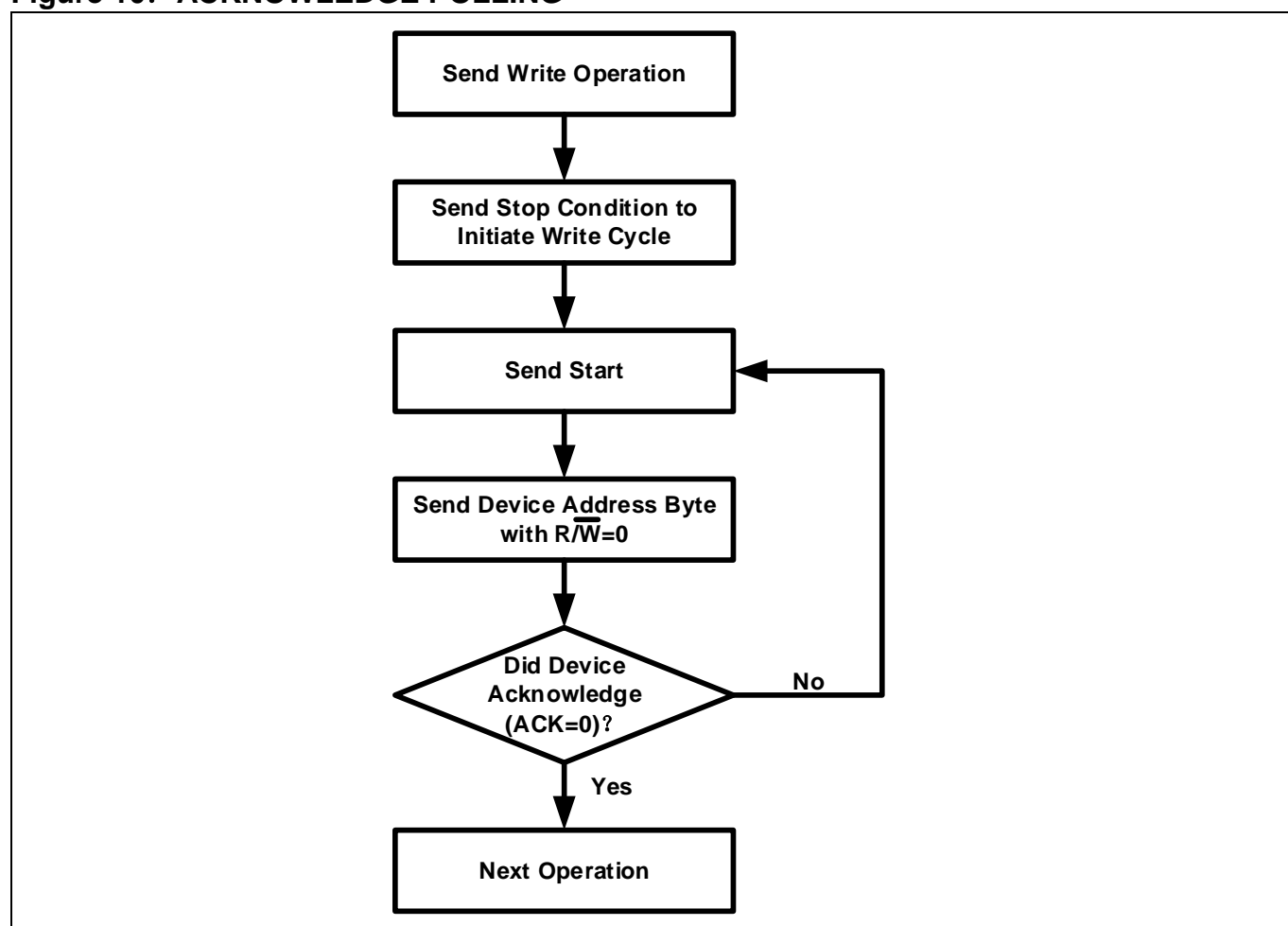
Figure 10. ACKNOWLEDGE POLLING
