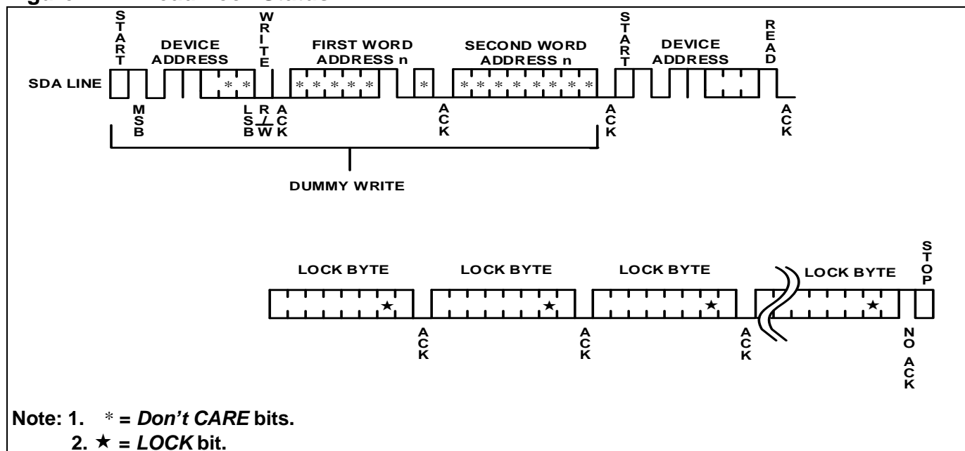
Figure 21. Read Lock Status
