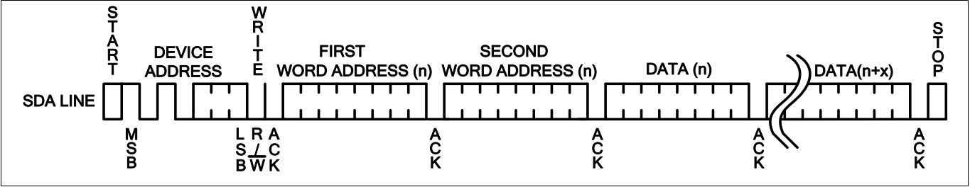
Figure 12. Page Write
