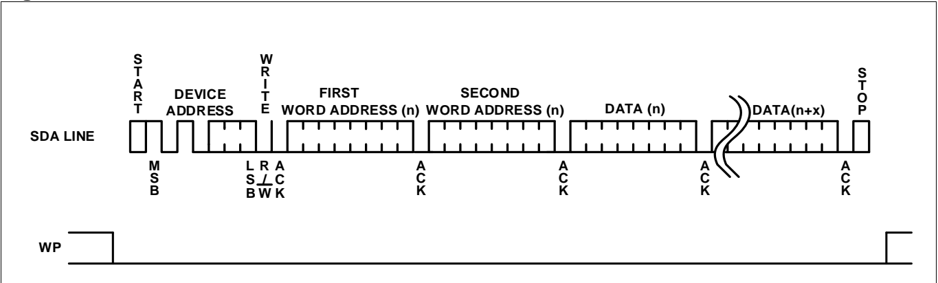
Figure 14. Non-Write-Protect Condition
