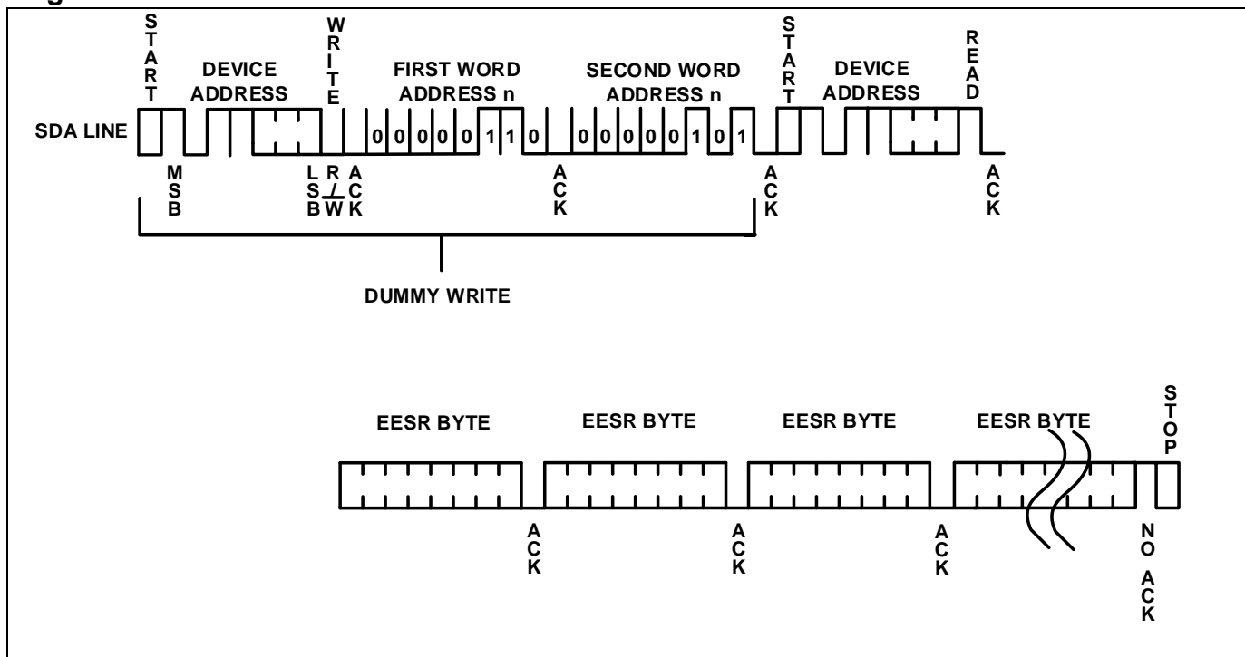
Figure 23. Read EESR
