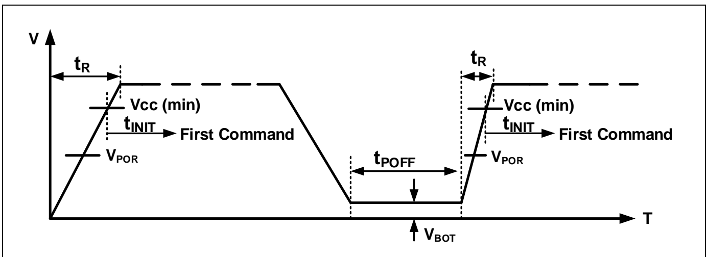
Figure 2. V_{CC} Ramp Up and Ramp Down
