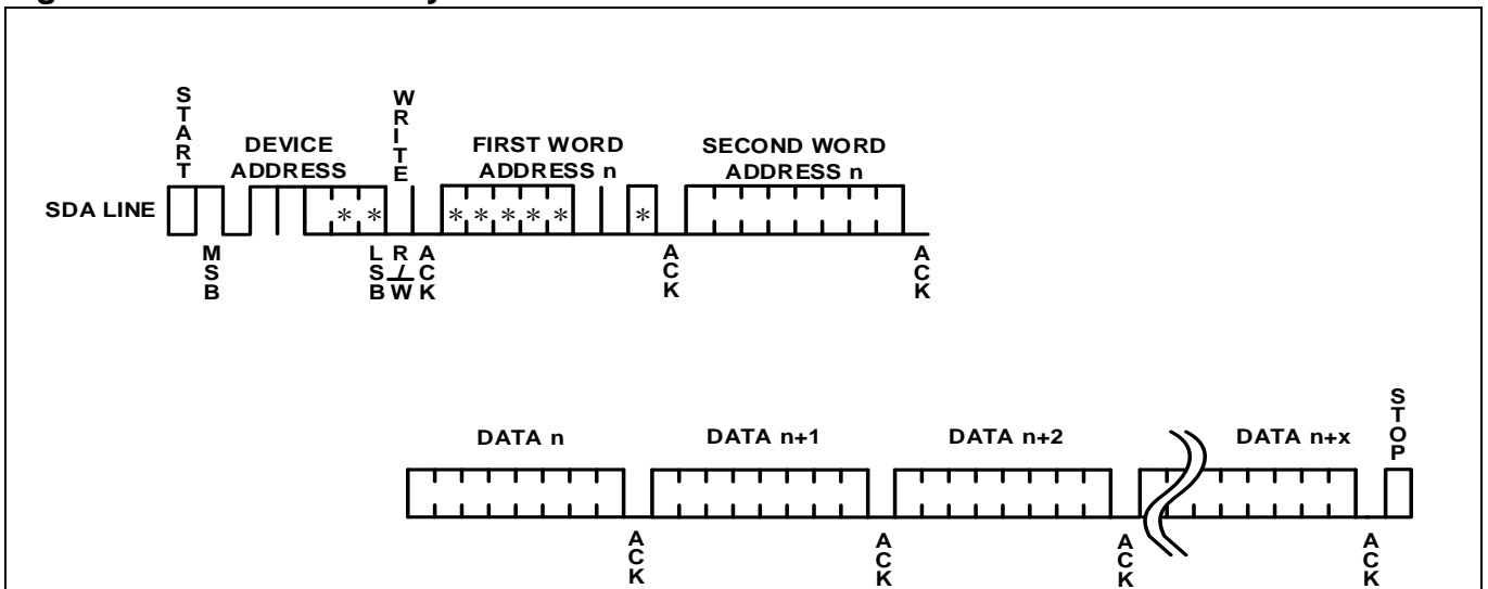
Figure 18. Write Security Sector
