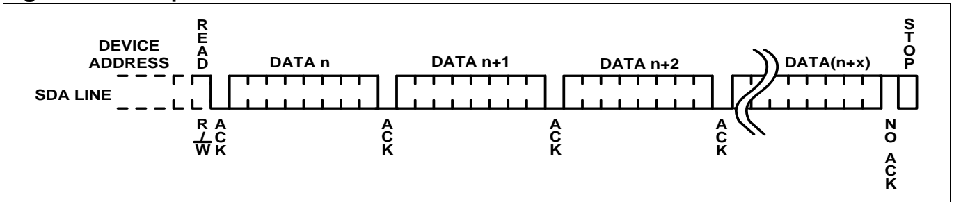
Figure 17. Sequential Read
