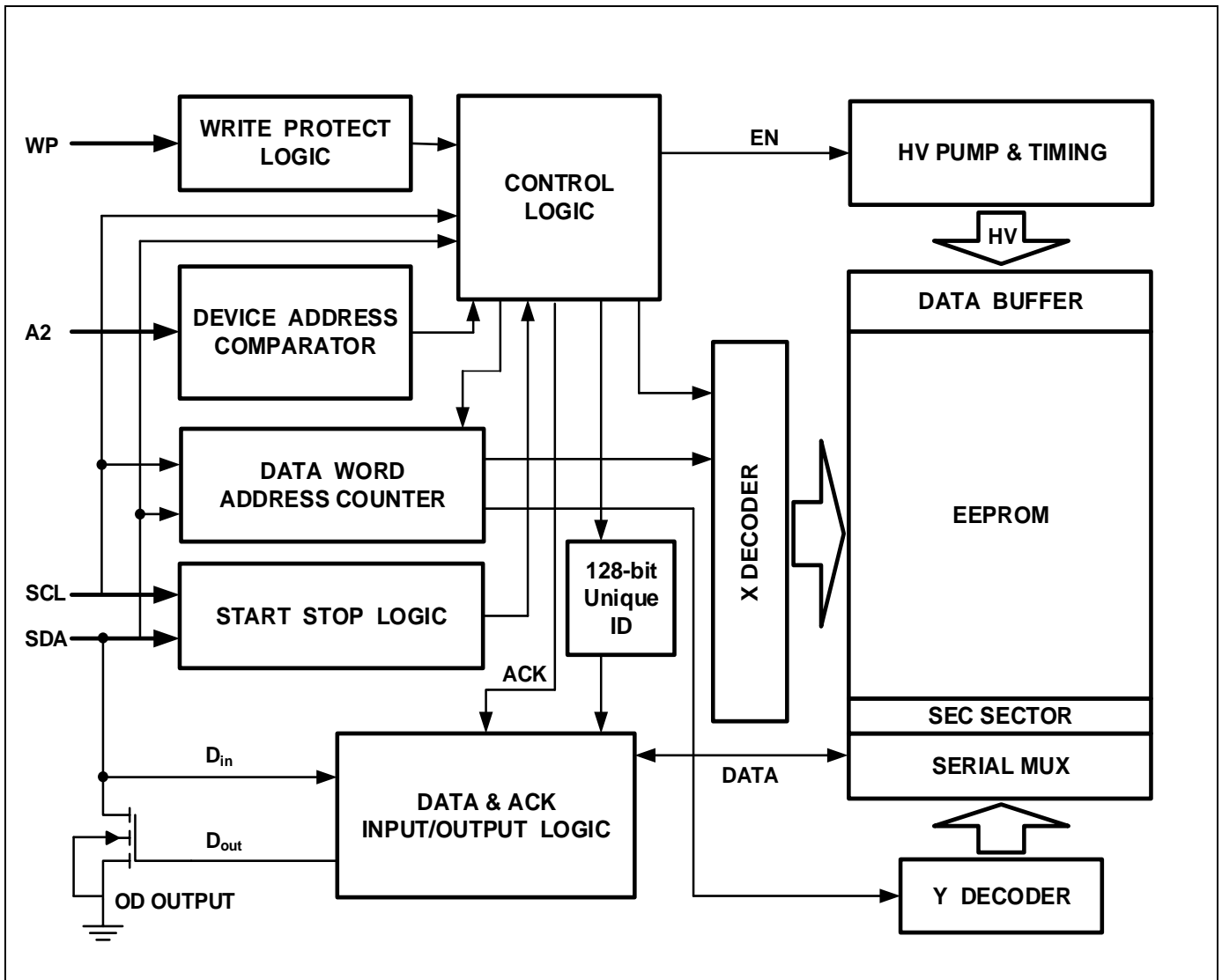
Figure 1. Block Diagram
