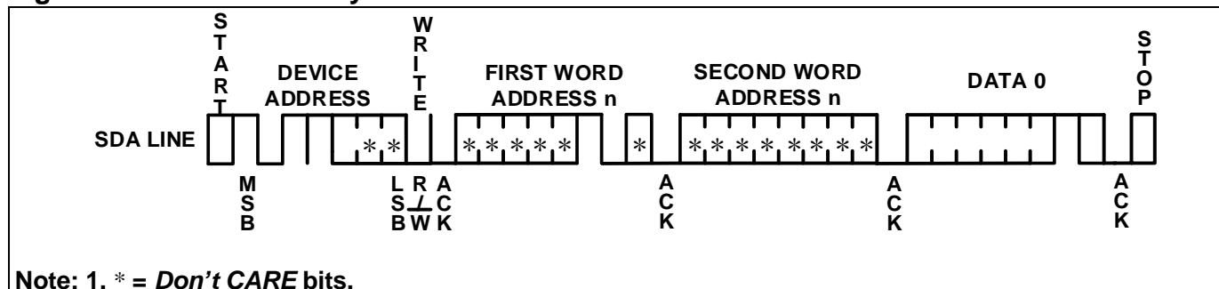
Figure 20. Lock Security Sector
