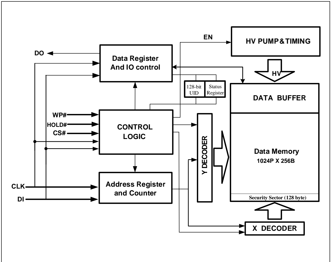
Figure 1 Block Diagram
