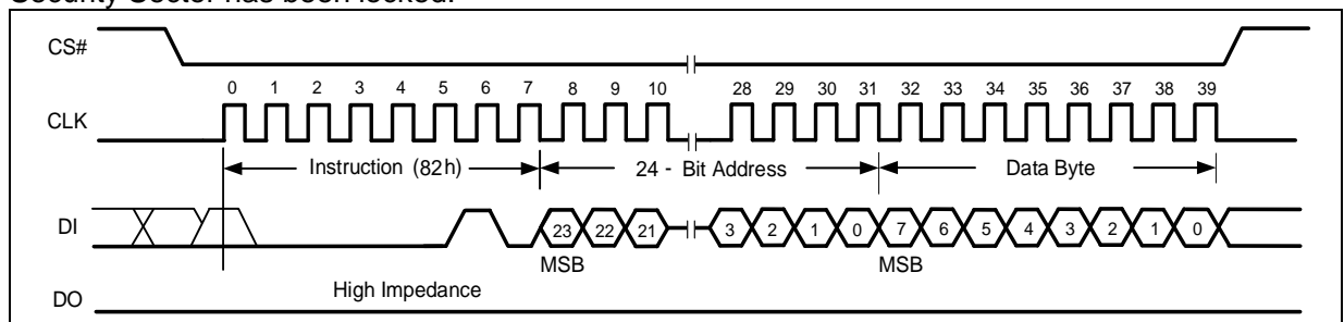
Figure 12 Write Security Sector Sequence
