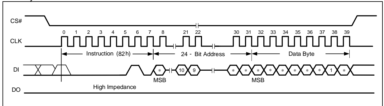
Figure 13 Lock Security Sector Sequence
