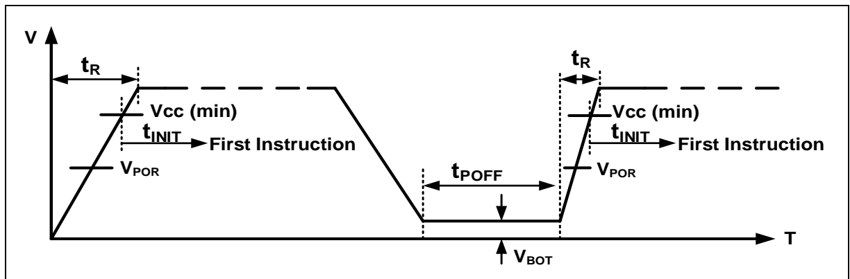
Figure 20. V_{CC} Ramp Up and Ramp Down
